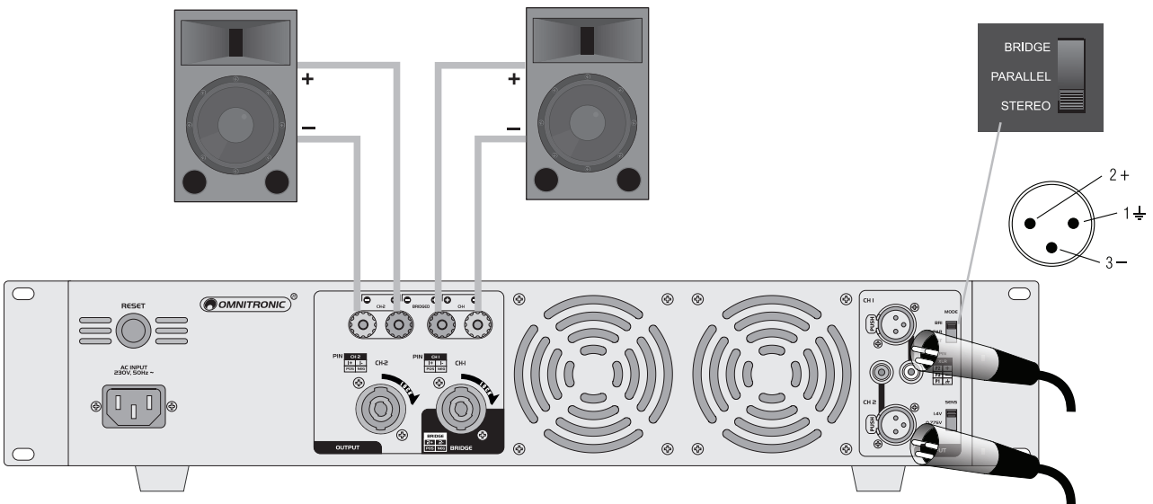
Fig. 2 Stereo wiring using the screw terminals
