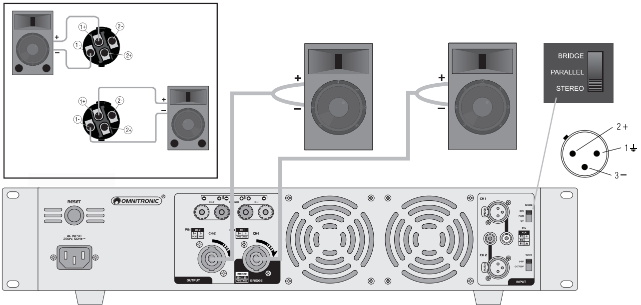
Fig. 1 Stereo wiring using the speaker connectors
