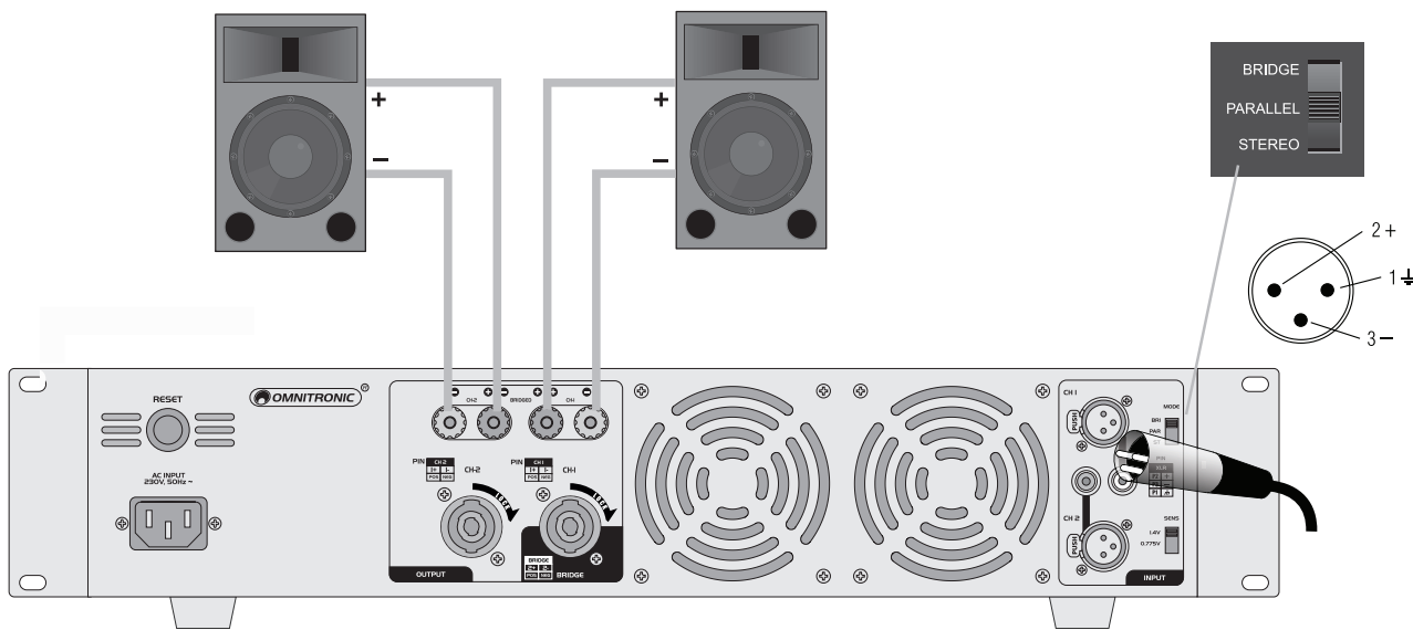
Fig. 4 Parallel wiring using the screw terminals
