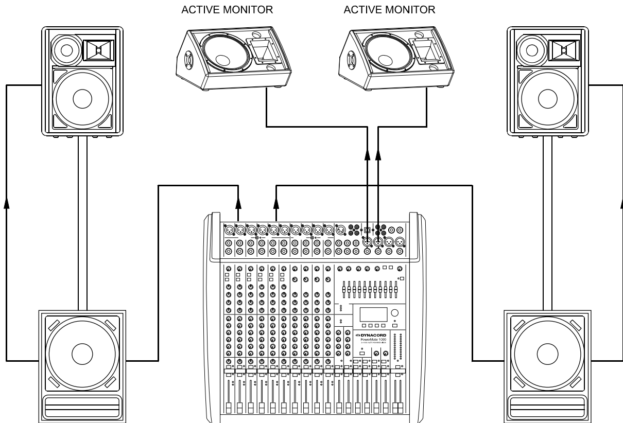
Illustration 5-1: Setting up a standard PA-system
